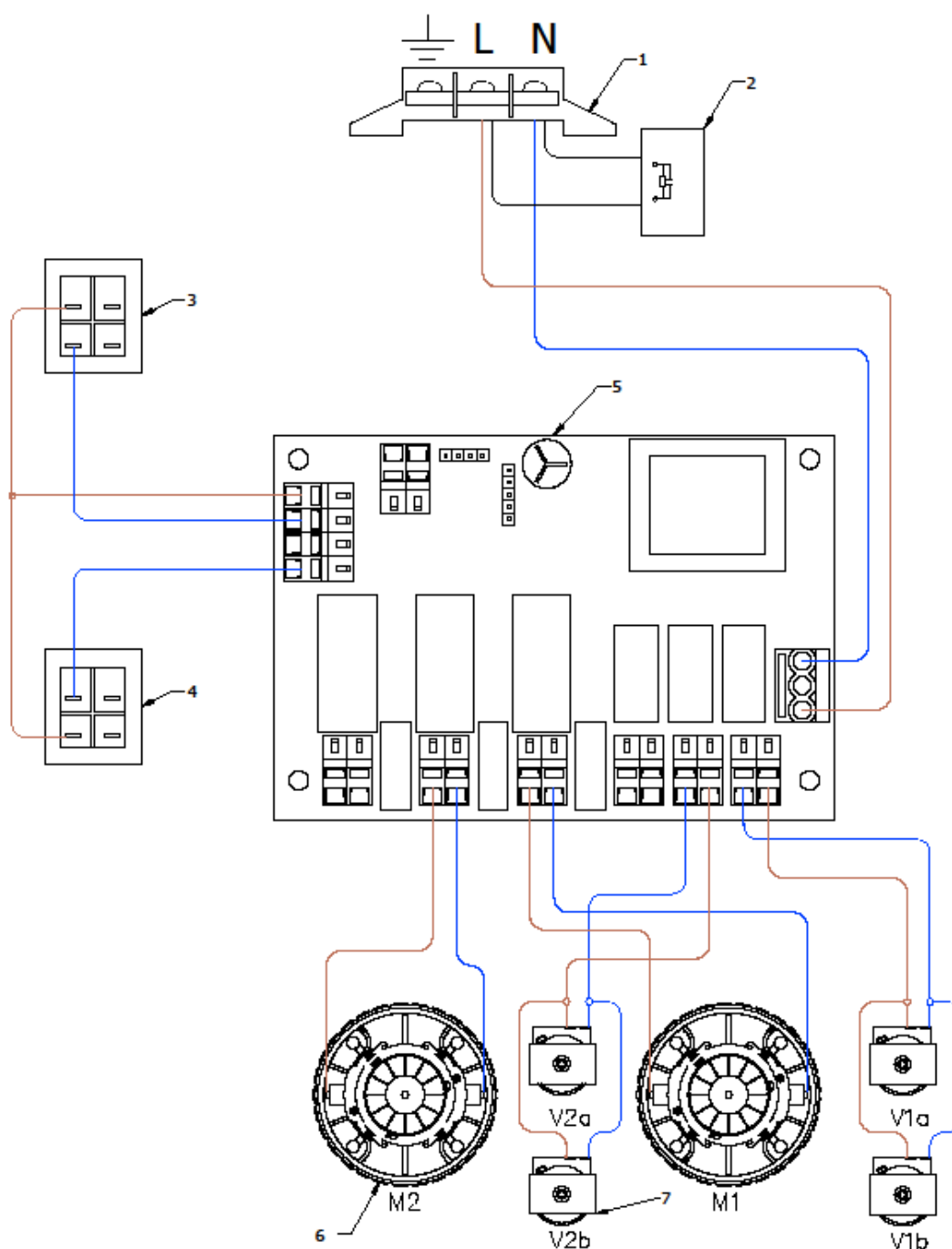
Parts Guide – Wiring Diagram W6
